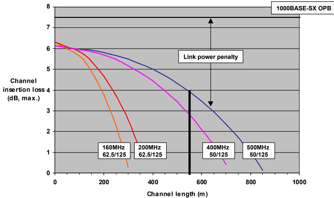
Figure 3 - 1000BASE-SX channel insertion loss
