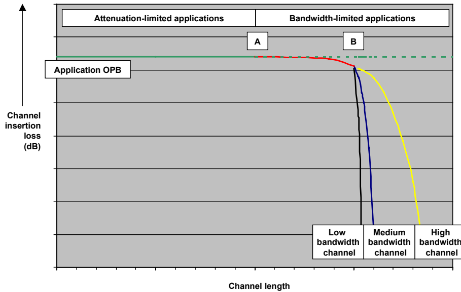
Figure 1 - General bandwidth-insertion loss characteristic
