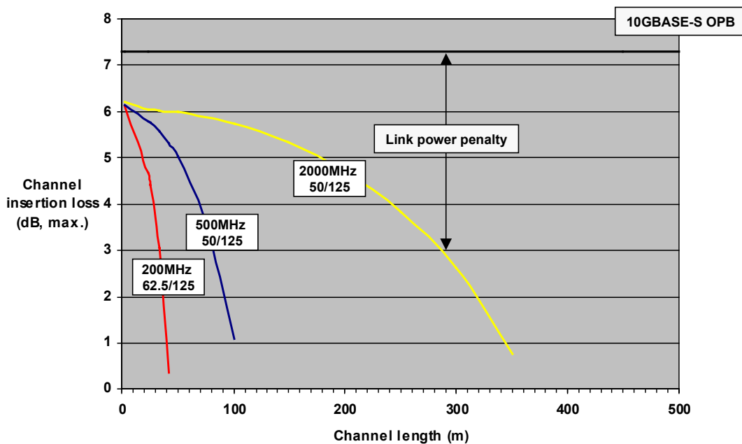
Figure 5 - 10GBASE-S channel insertion loss
