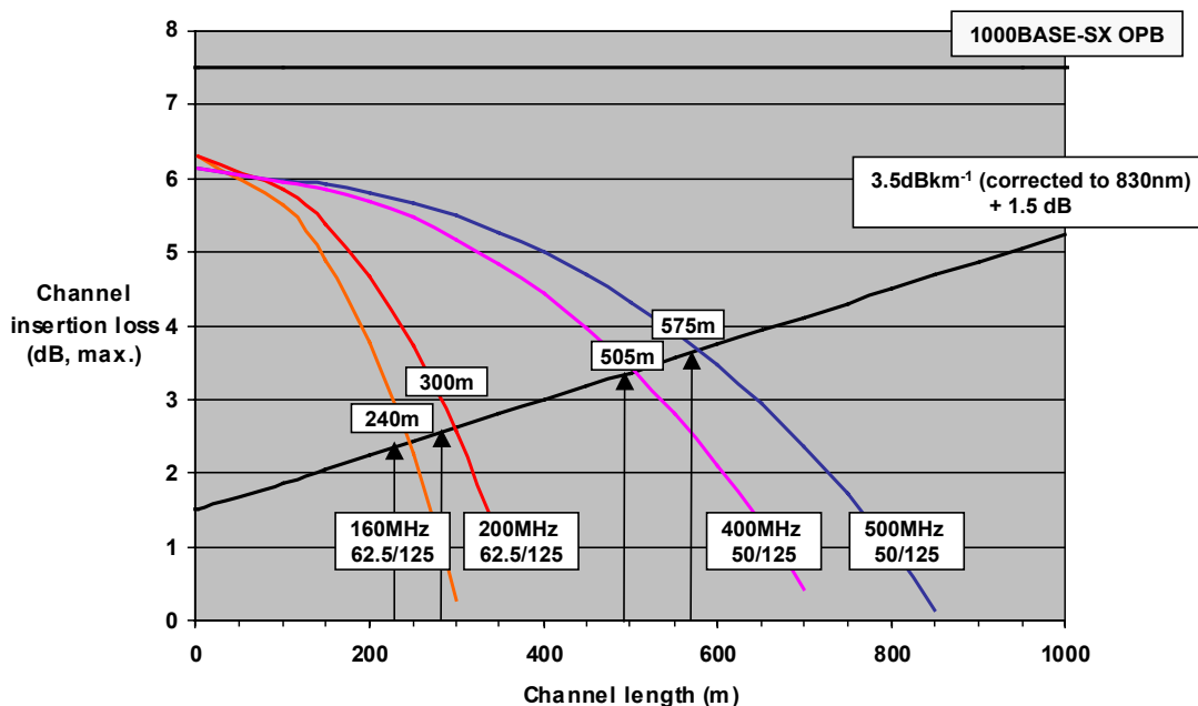
Figure 4 - 1000BASE-SX channel insertion loss and zero margin lengths
