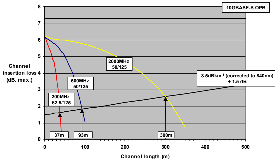
Figure 6 - 10GBASE-S channel insertion loss and zero margin lengths
