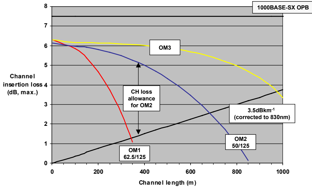
Figure 8 - Connecting hardware (CH) loss allowances for OM1, OM2 and OM3 cabled optical fibres for 1000BASE-SX
