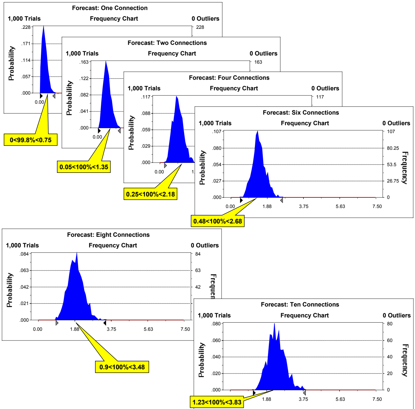
Figure 11 - Predictive Monte Carlo modelling of connection loss
