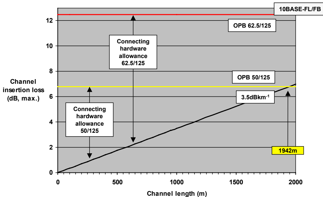
Figure 2 - 10BASE-FL/FB insertion loss characteristic
