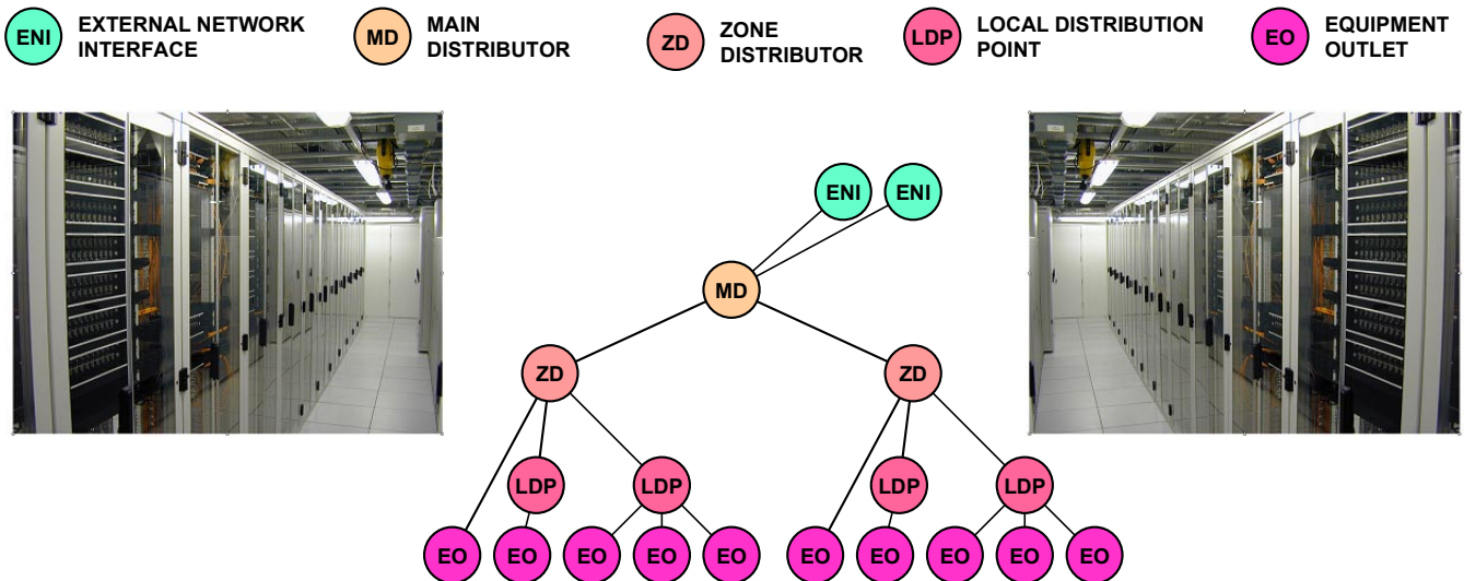
Figure 10 - Cabling structure in data centres according to EN 50173-1
