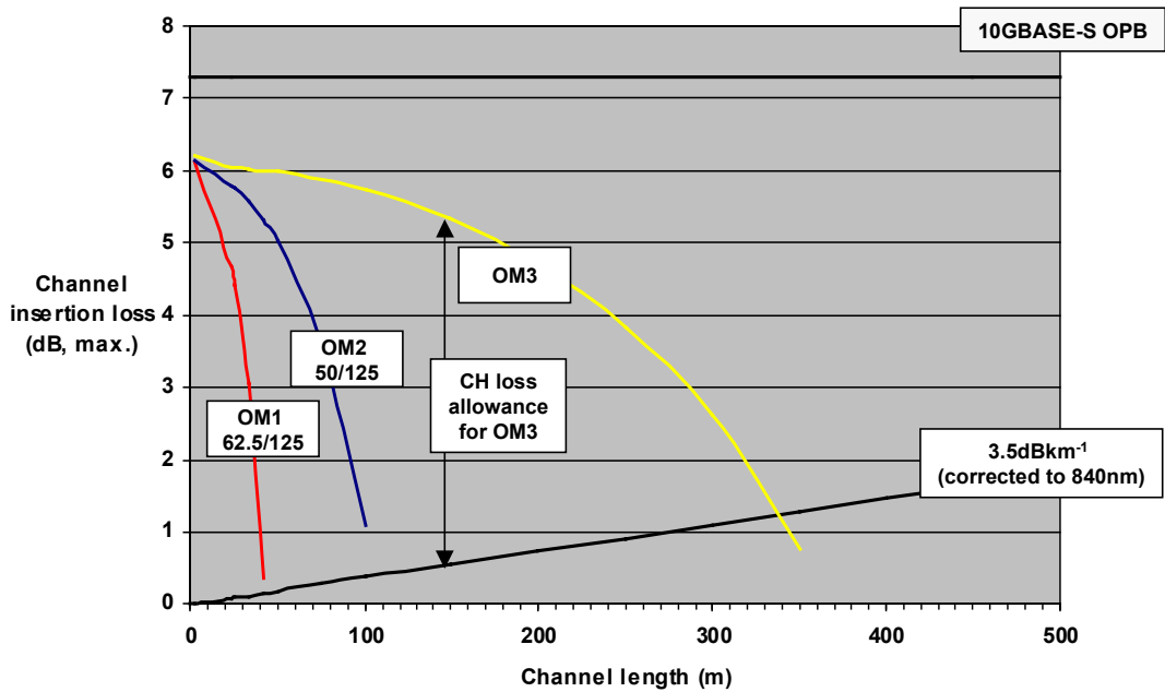
Figure 9 - Connecting hardware (CH) loss allowances for OM1, OM2 and OM3 cabled optical fibres for 10GBASE-S
