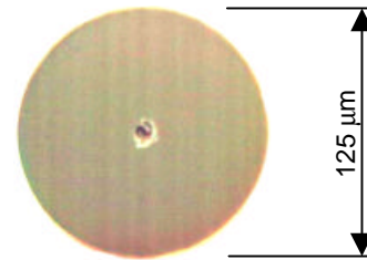
Fig. 1: Burnt singlemode fiber
