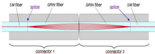
Fig.4: Expanded beam connectors based on gradient index fibers
